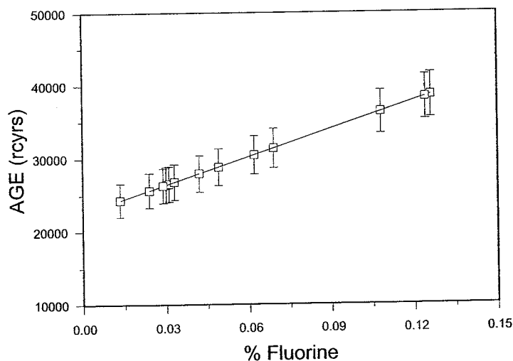
Figure 4. Predicted age (with 1 sigma confidence limits) of 13 specimens of Geocapromys brownii from Red Hills Fissure, Jamaica.
