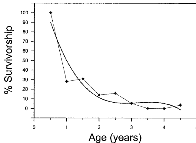
Figure 2. Survivorship curve for late Pleistocene Geocapromys brownii collected from Red Hills Fissure, Jamaica.
