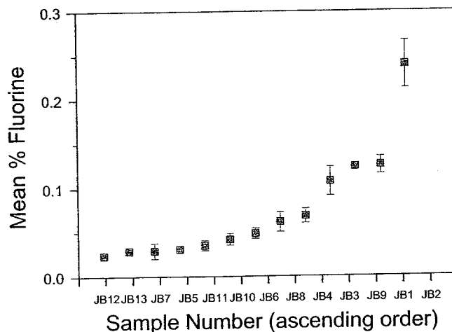
Figure 3. Fluorine content (percentage by dry bone mass) of 13 samples of Geocapromys brownii bone from Red Hills Fissure, Jamaica.
